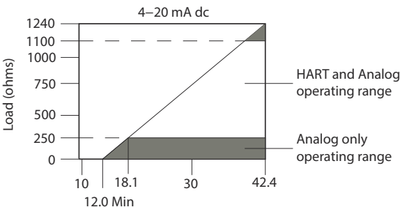
Figure 2: Load Limitations
