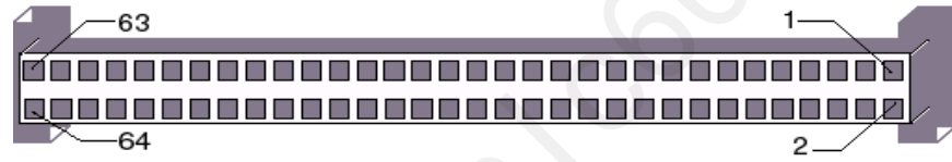
Figure A-5 V7768 PCI-X PMC Site Connector (J12)
