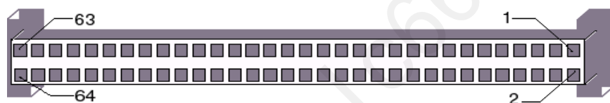
Figure A-10 Mezzanine PCI-X PMC Site Connector (J12)
