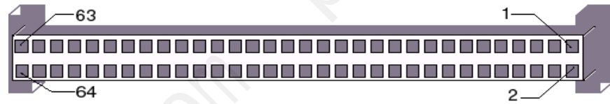
Figure A-4 V7768 PCI-X PMC Site Connector (J11)
