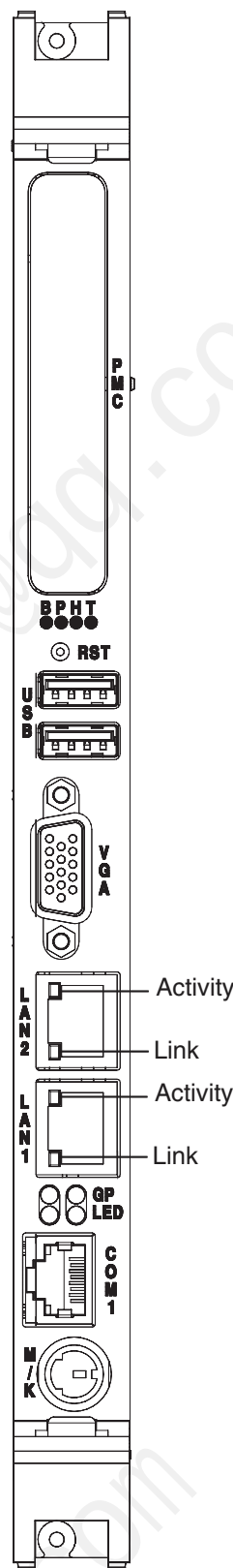
Figure 1-7 V7768 Front Panel Layout
