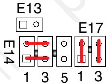
RS422 w/Termination
