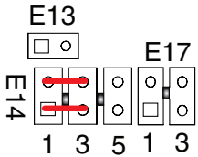
RS422 w/o Termination
