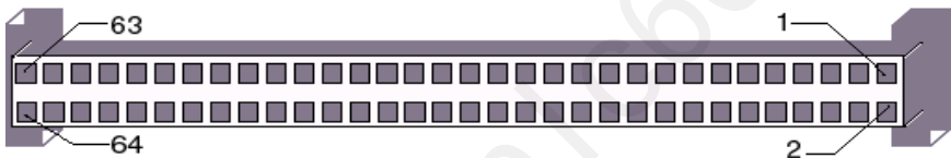
Figure A-7 Mezzanine PCI-X PMC Site Connector (J14 )
